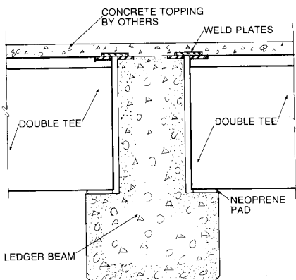
DOUBLE TEE BEARING ON LEDGER BEAM
