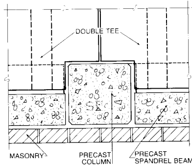
DOUBLE TEE CUT-OUT AT PRECAST COLUMN
