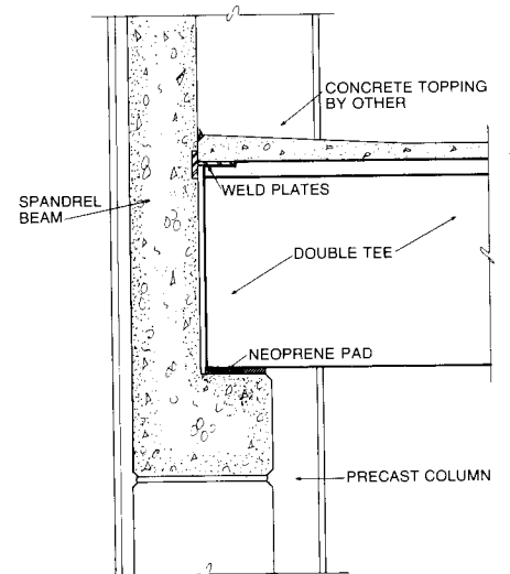
DOUBLE TEE ON SPANDREL BEAM
