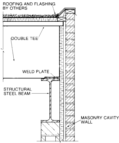
DOUBLE TEE BEARING ON STRUCTURAL BEAM
