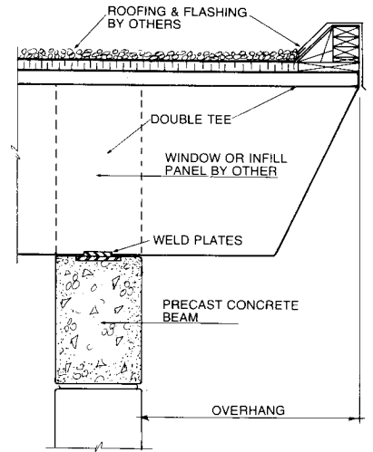
DOUBLE TEE ON CONCRETE BEAM
