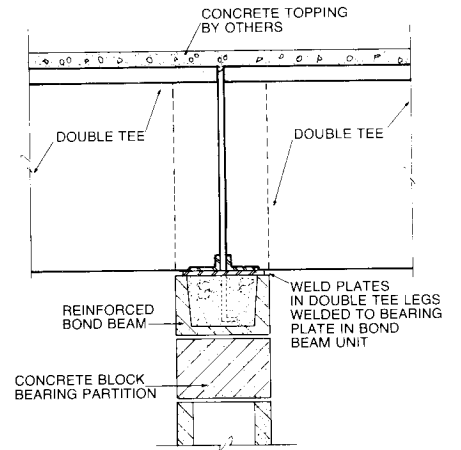
DOUBLE TEES BEARING ON MASONRY WALL
