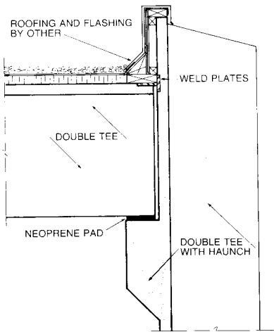
DOUBLE TEE ROOF AND WALL PANELS
