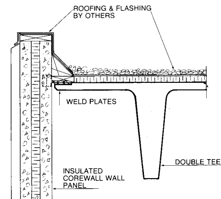
DOUBLE TEE RUNNING PARALLEL TO COREWALL PANEL
