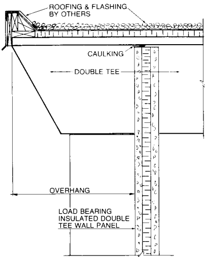
DOUBLE TEE ROOF AND WALL PANELS
