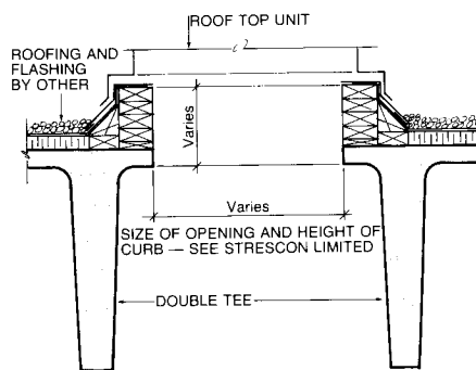
DOUBLE TEE WITH FRAMED OPENING
