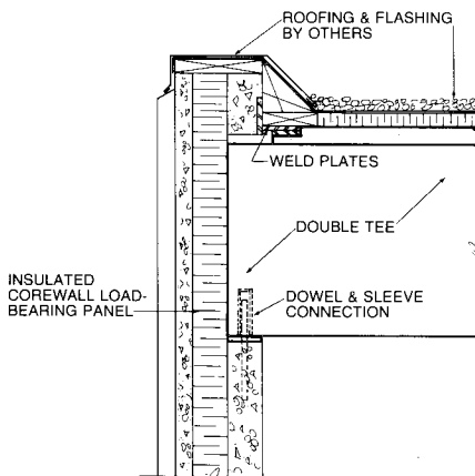
DOUBLE TEE BEARING ON COREWALL
