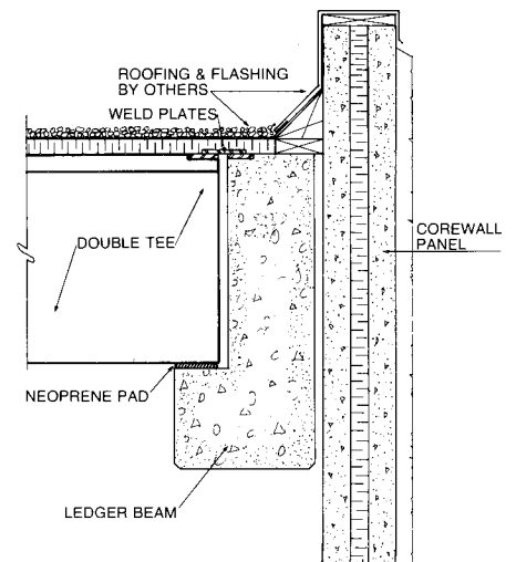
DOUBLE TEE BEARING ON LEDGER BEAM
